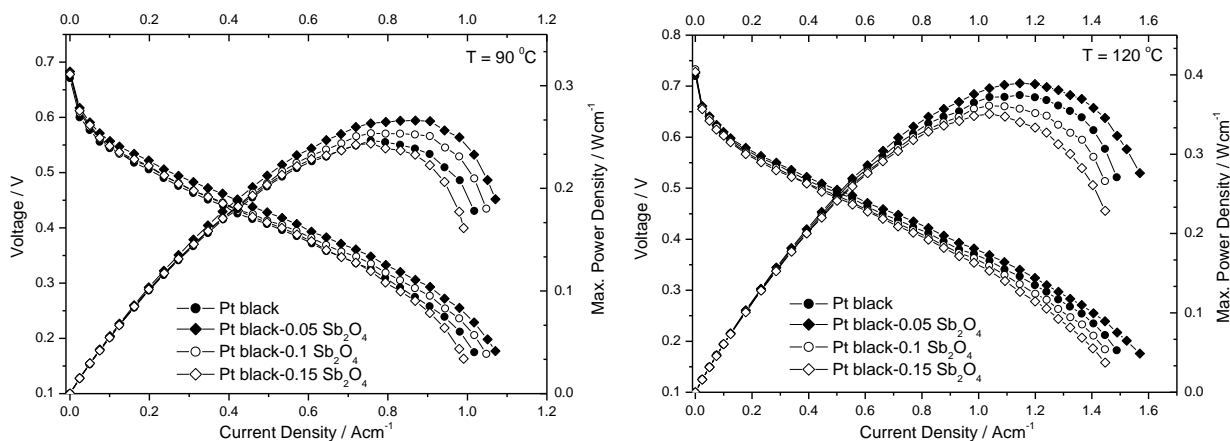
Fig. 1 The polarization curves compared to pure Pt catalyst operated at (a) 90^\circ\text{C} and (b) 120^\circ\text{C} .
